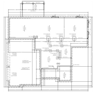
FOUNDATION PLAN
